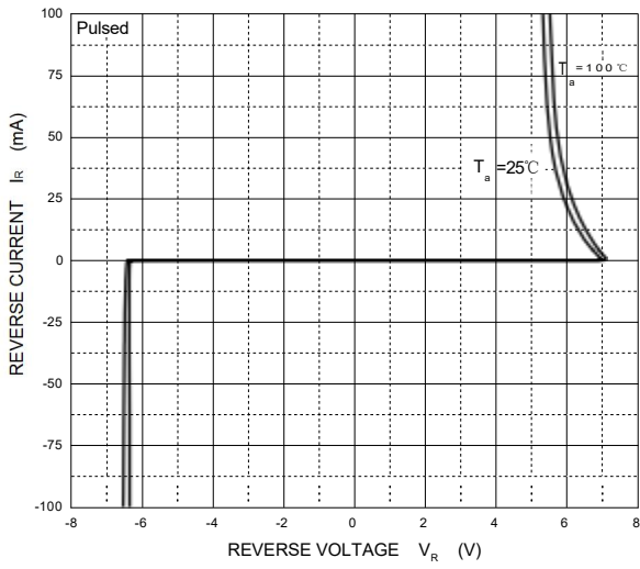
Reverse Characteristics
